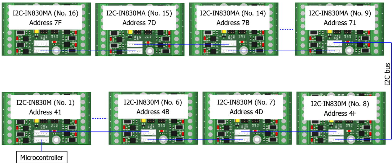
Figure 6: Boards on a bus
