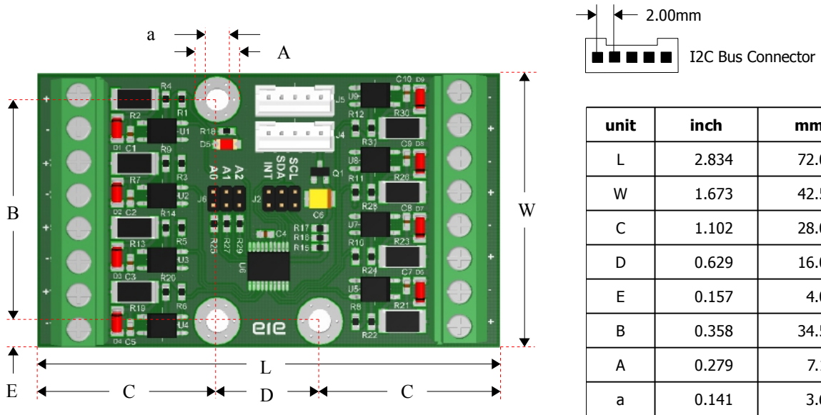
Figure 9: Dimensions
