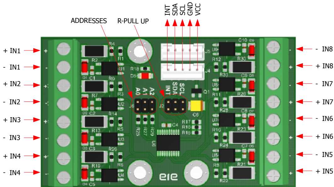
Figure 2: Board Diagram
