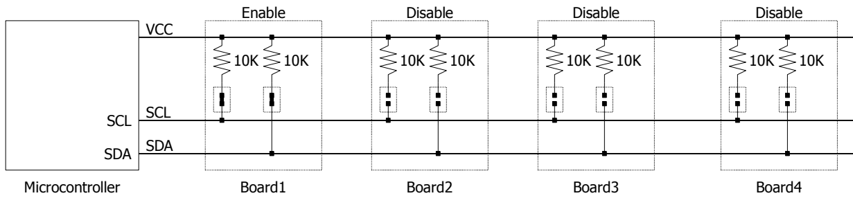
Figure 3: I2C bus pull-up resistors
