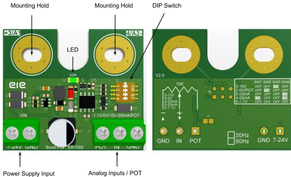
Figure 1: Board diagram
