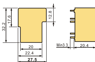
CMP7 Demensions
